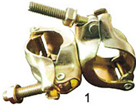
1 JIS Type Pressed Fixed Coupler 60.5x60.5mm 48.6x48.6mm
